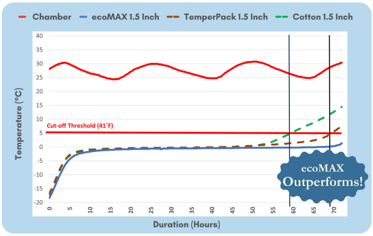
Test: ISTA 7E Summer Profile using 12 Cube Cartons (9#s Frozen gels)
